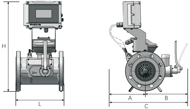
图3-2 TBQM-□/FCM
