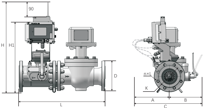
图3-6 TBQM-□/FCC-III-□-B
