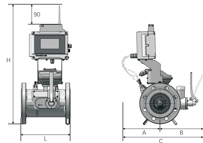
图3-3 TBQM-□/TFC-B
