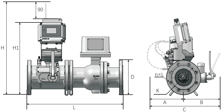
图3-8 TBQM-□/FCC-S-□-M
