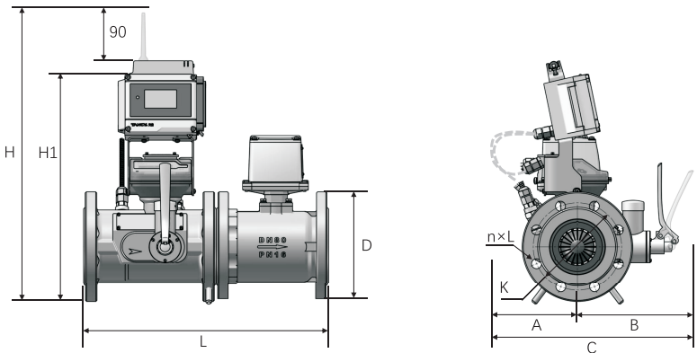
图3-9 TBQM-□/FCC-S-□-C
