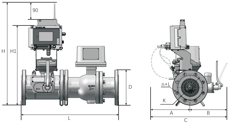
图3-7 TBQM-□/FCC-III-□-M
