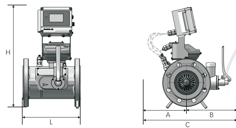
图3-4 TBQM-□/FCM-V
